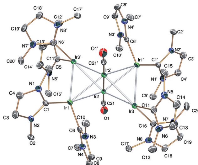
Figure 1. ORTEP diagram of the cationic portion of compound 2 . Thermal ellipsoids are shown at 50%. Hydrogen atoms, two \text{BAR}_\text{F} counterions, and a pentane solvent molecule have been omitted for clarity. The metal hydrides were not located in the Fourier map.
